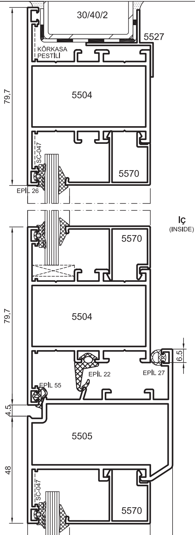
Detay Detail 5
