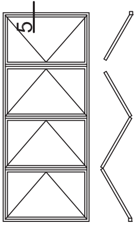
KATLANIR SÜRME KAPI Folding Sliding System Detail
