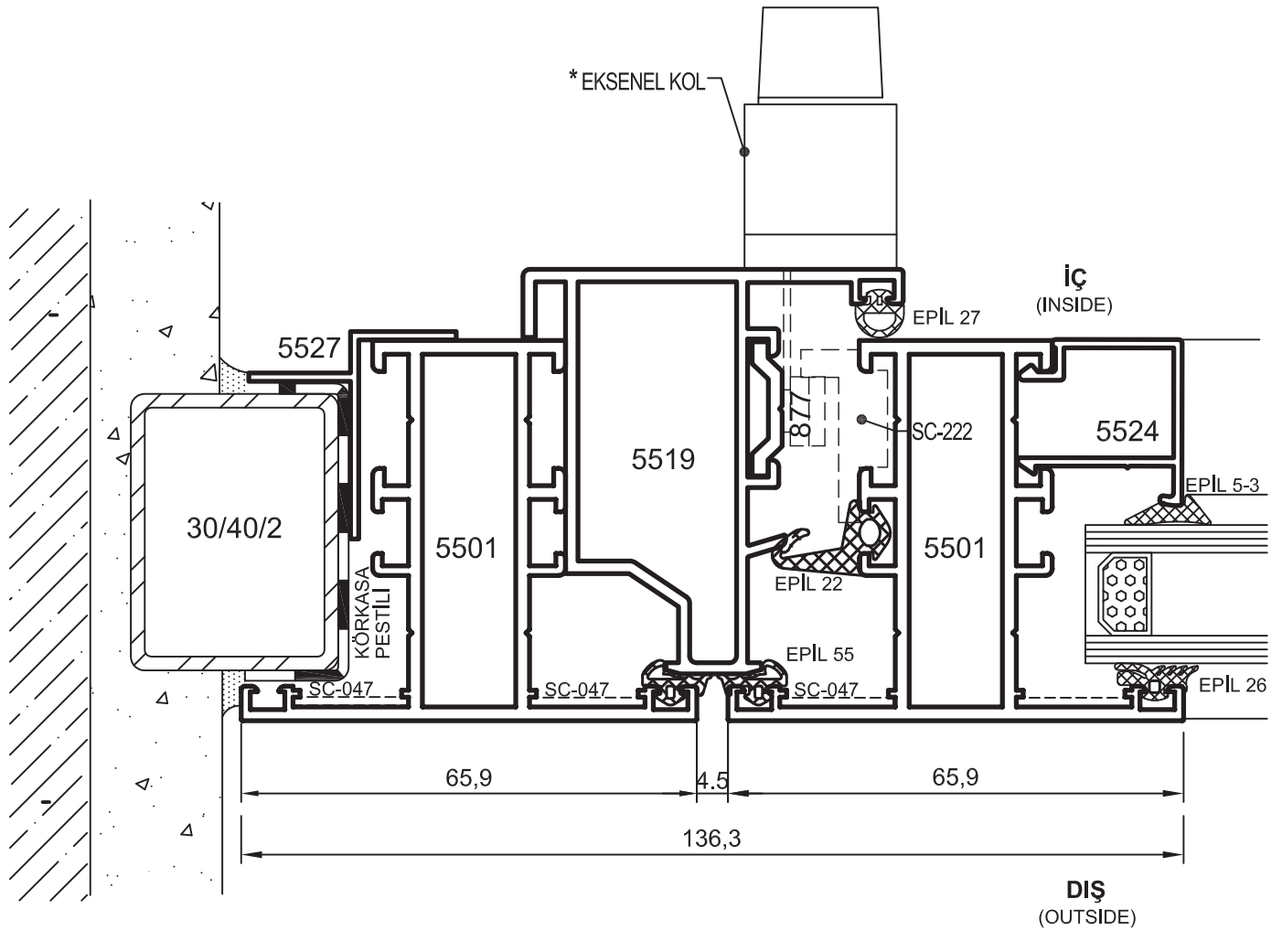
Detay 1 Detail 1
