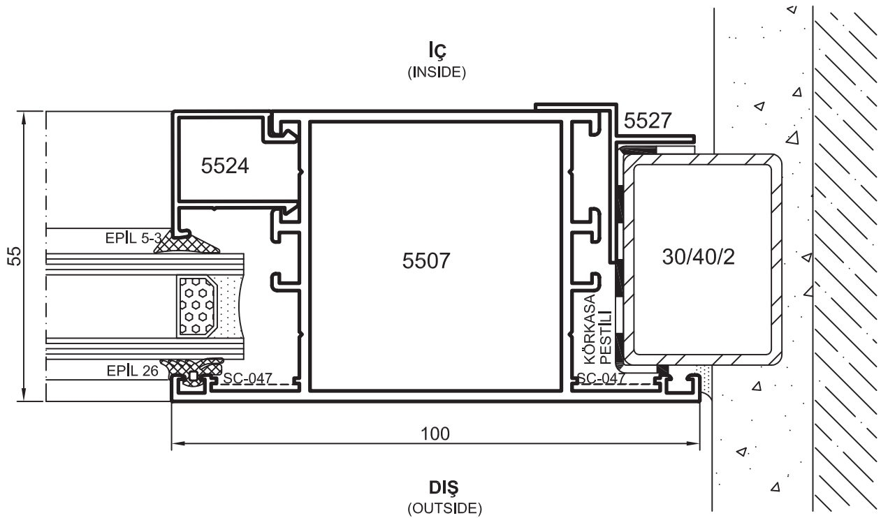
Detay 4 Detail 4
